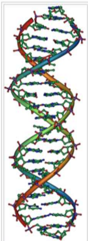
DNA, the molecular basis for biological inheritance. Each strand of DNA is a chain of nucleotides, matching each other in the center to form what look like rungs on a twisted ladder.
