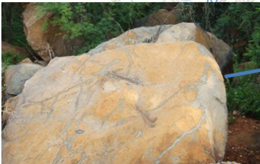
Dolerite intrusion through Granite
